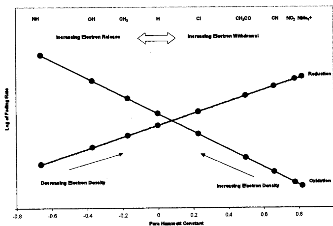
Figure 3. Schematic plot of the logarithm of fading rate vs. the Hammett constant.
