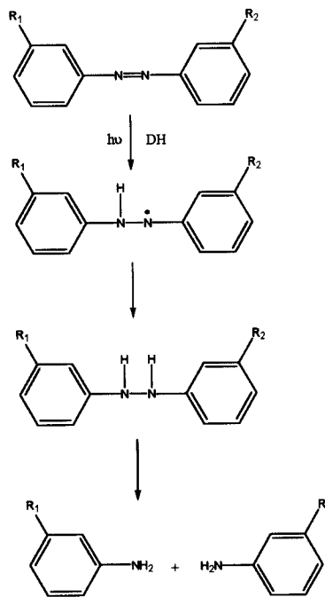
Figure 1. Reduction mechanism for azo dyes.
