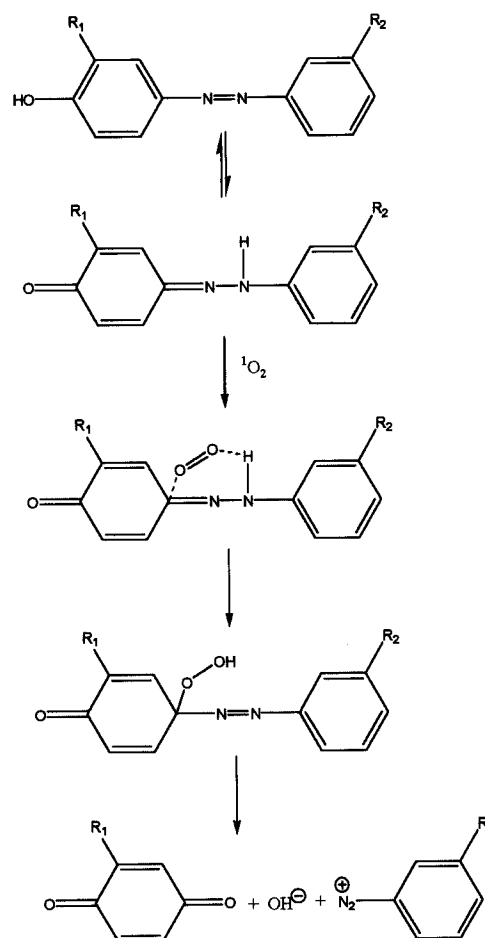
Figure 2. Oxidation mechanism for azo dyes.
